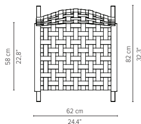
01713 - Rocking chair
